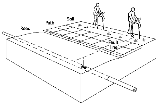
Figure 8.2: Locating faults with the locator and A-frame
